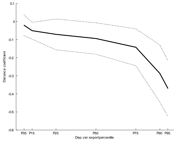
Figure 10: The impact of trade costs on the export distribution.
