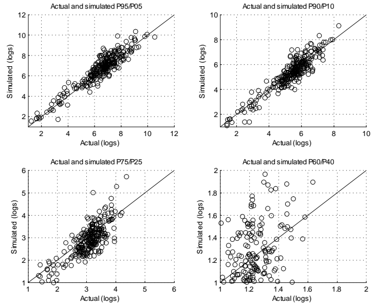
Figure 9: Model evaluation. Empirical and simulated percentile ratios.
